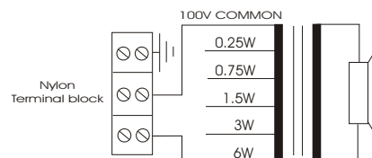
PBC6/T Circuit Diagram
