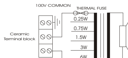
PBC6/TC Circuit Diagram
