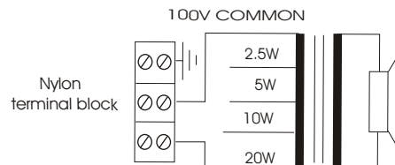
PH20/T Circuit diagram
