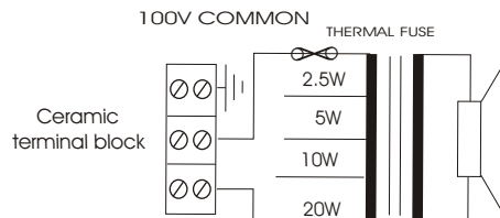
PH20/TC Circuit diagram
