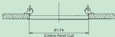
Mounting Bracket To Ceiling Panel
